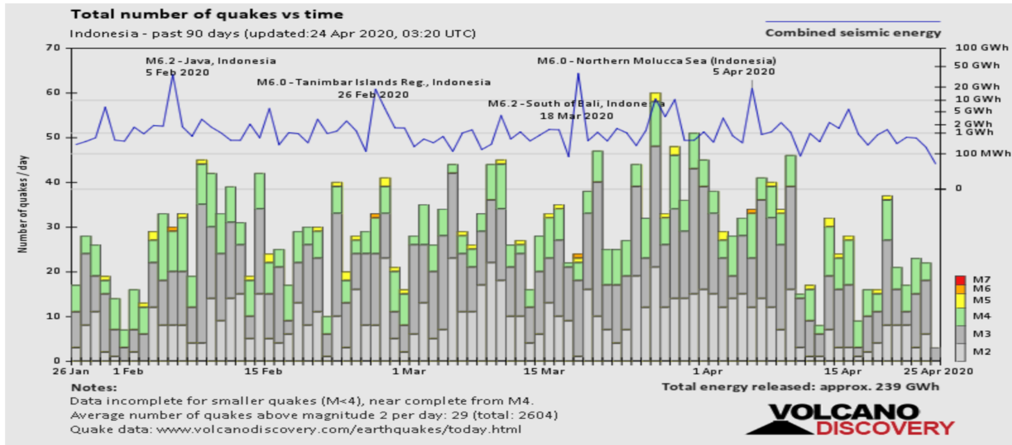
Number of quakes vs time
